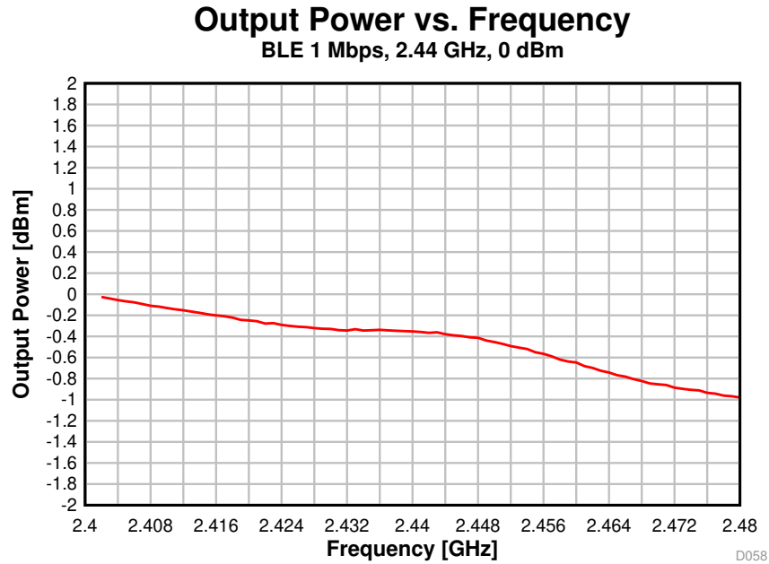
Figure 5-18. Output Power vs. Frequency (BLE 1 Mbps, 2.44 GHz)
