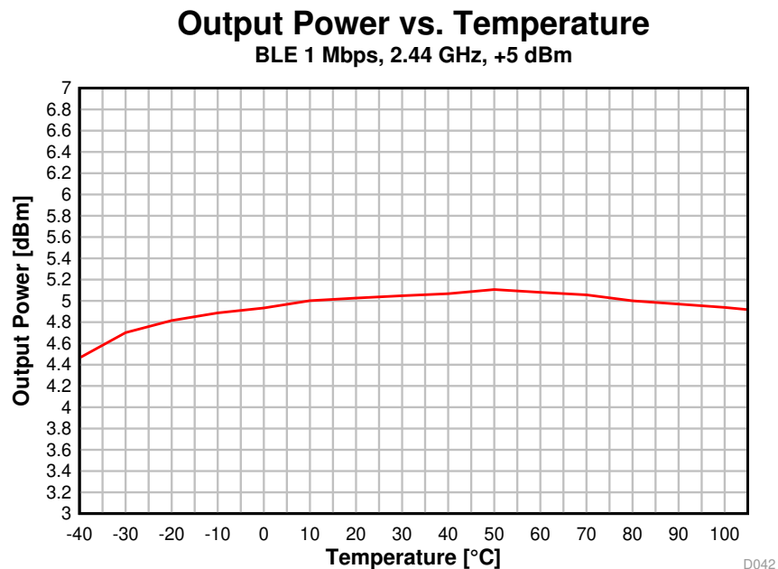
Figure 5-15. Output Power vs. Temperature (BLE 1 Mbps, 2.44 GHz, +5 dBm)
