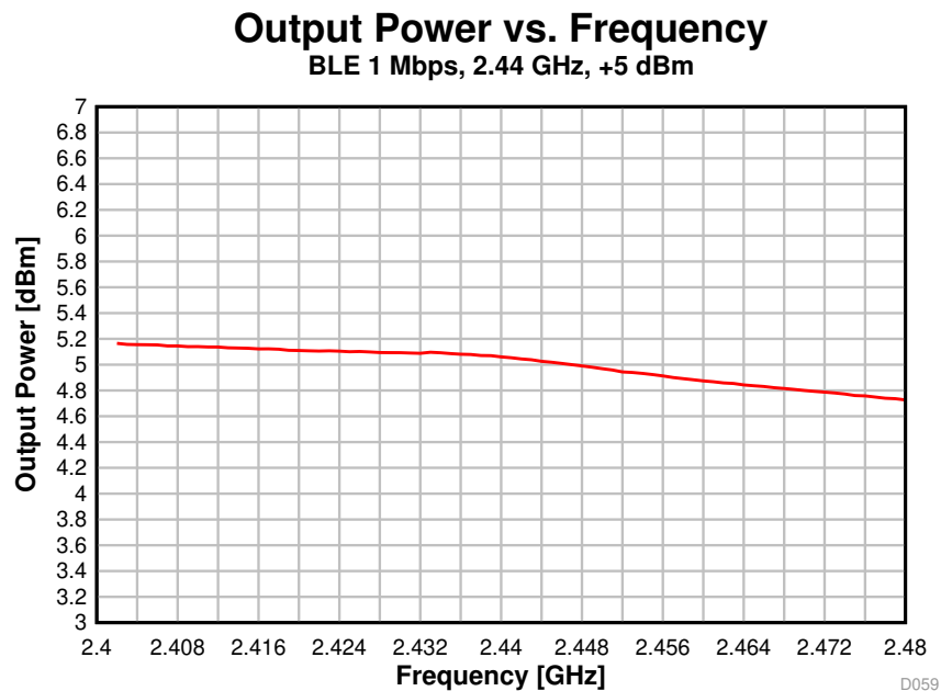
Figure 5-19. Output Power vs. Frequency (BLE 1 Mbps, 2.44 GHz, +5 dBm)
