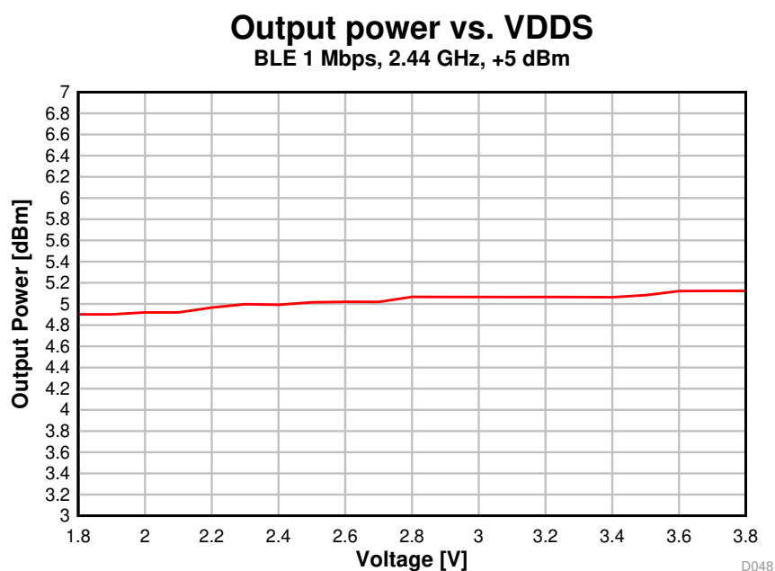
Figure 5-17. Output Power vs. Supply Voltage (VDDS) (BLE 1 Mbps, 2.44 GHz, +5 dBm)
