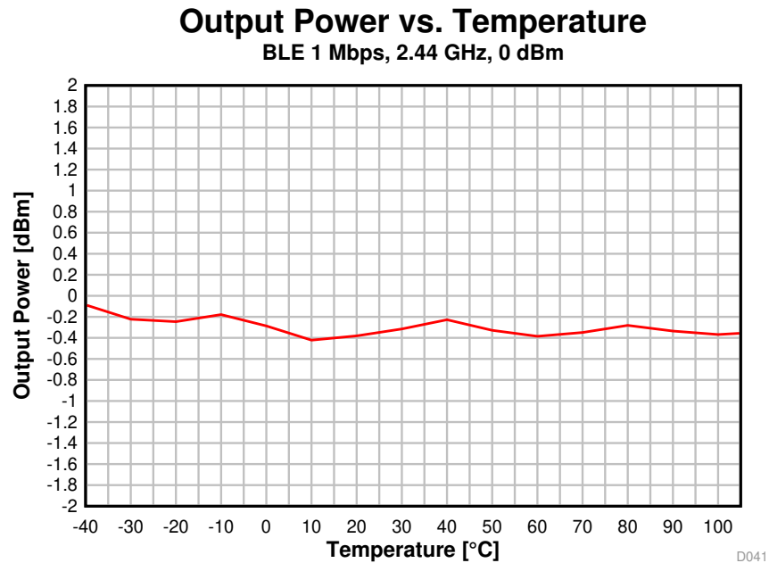
Figure 5-14. Output Power vs. Temperature (BLE 1 Mbps, 2.44 GHz)
