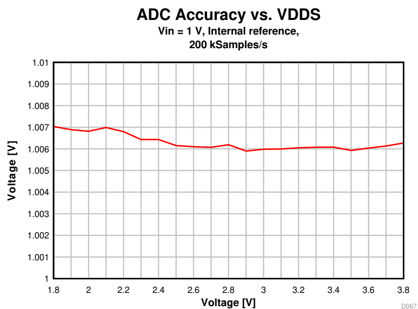
Figure 5-25. ADC Accuracy vs. Supply Voltage (VDDS)
