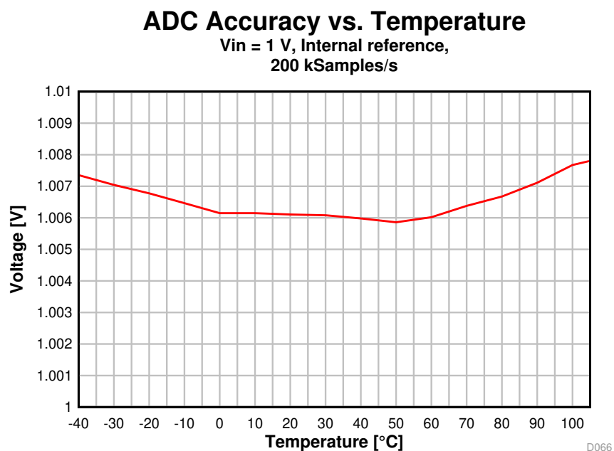
Figure 5-24. ADC Accuracy vs. Temperature
