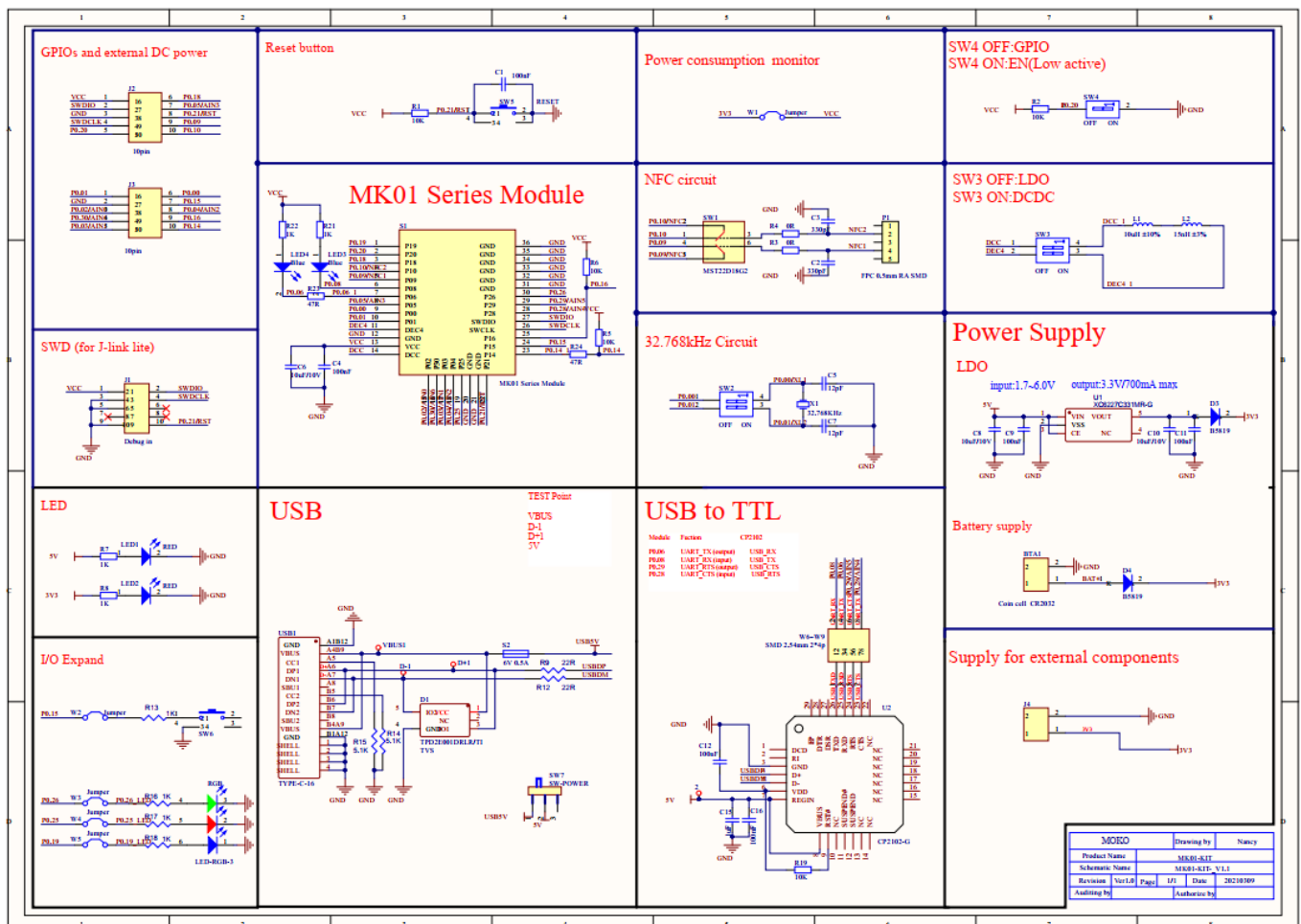
Figure 4: Schematic of MK01-KIT
