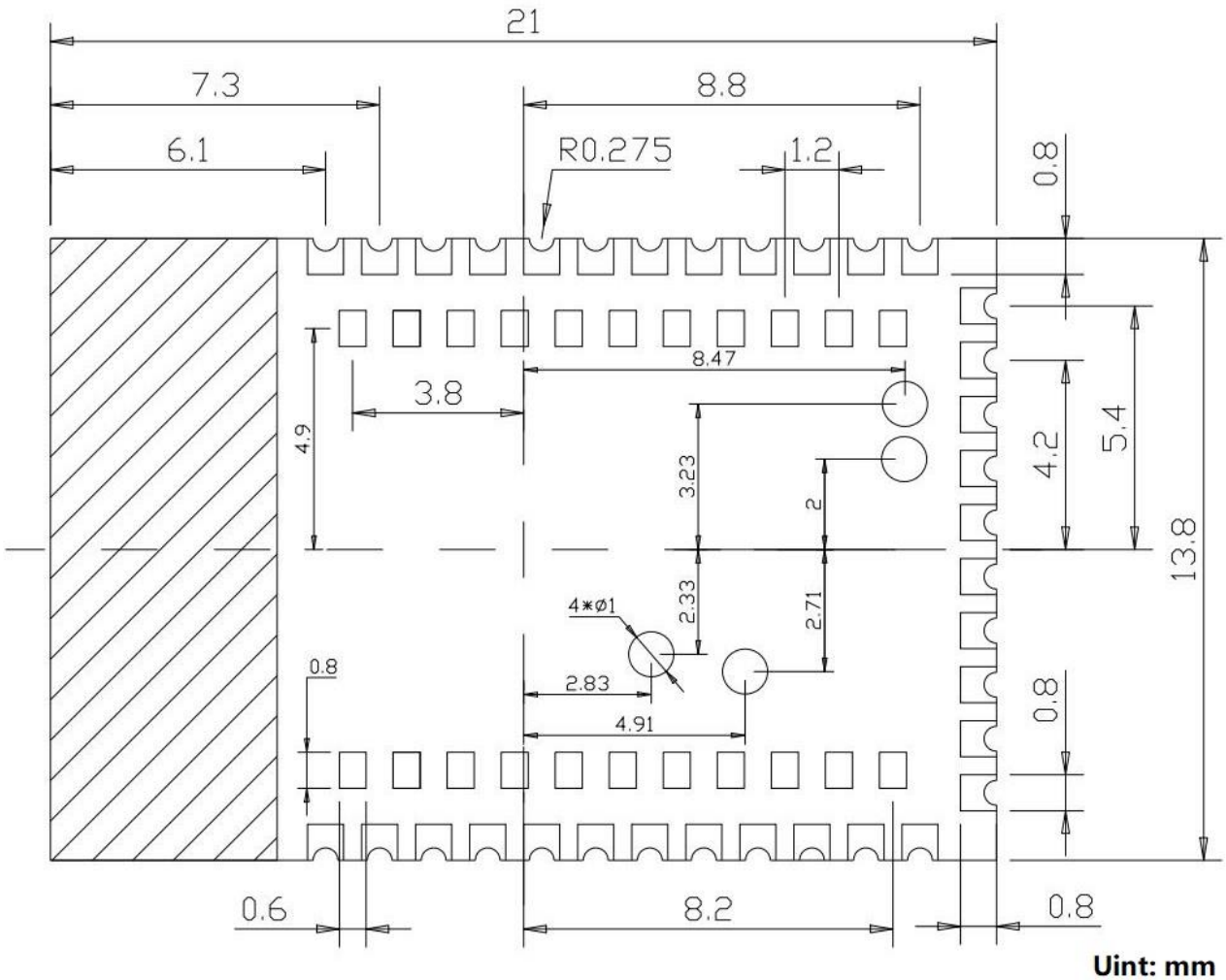
MK08 PCB land pads (TOP View)
